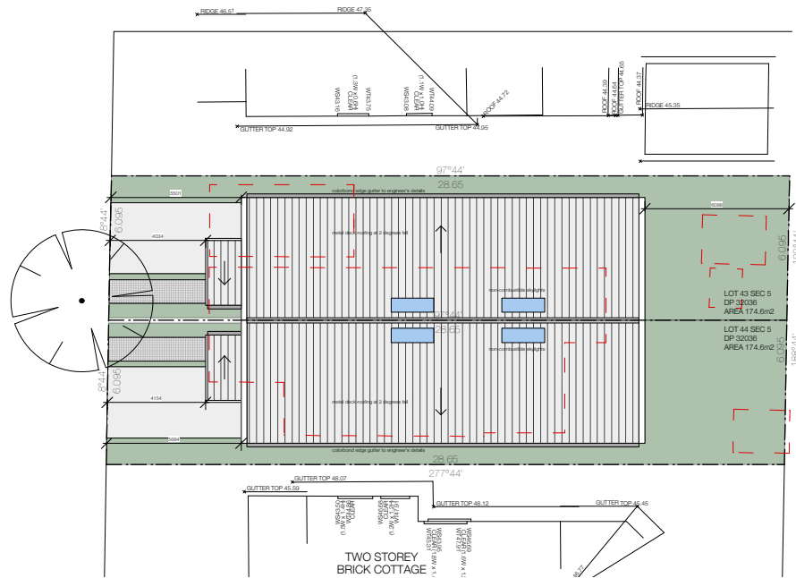
SITE PLAN 1:200 @ A3
